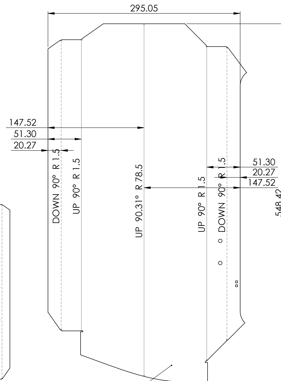
TOD6-11 v1.2R, SM-FLAT-PATTERN
